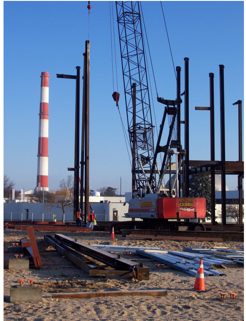
Setting Column
