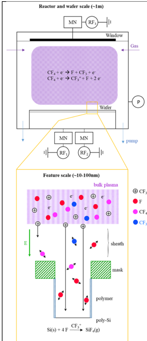
Figure 1: Si etching using a \text{CF}_4 plasma.
