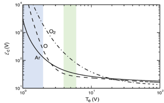
Collisional energy loss per electron-ion pair created as a function of electron temperature [164]
