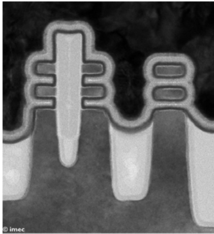
TEM image of IMEC 17 nm forksheet FETs, featuring atomic scale processes alongside both vertical and horizontal anisotropic etch processes. [169]
