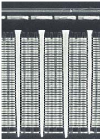
Figure 2: High aspect ratio structures fabricated using plasma etching. [173]
