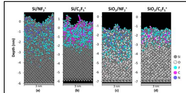
Figure 4-4: Fundamental Plasma-Surface Interactions by Molecular Dynamics. The interaction of plasma activated species and sheath accelerated ions with wafers (and plasma facing surfaces in the chamber) is at the heart of semiconductor fabrication. Molecular dynamics (MD) simulation is a first principles technique able to derive fundamental reaction probabilities and products, and predict the evolution of small features. The top image shows MD results for Si and \text{SiO}_2 after bombardment by 500 eV \text{NF}_2^+ and \text{C}_2\text{F}_5^+ ions. The bottom image shows the desorbed products following \text{C}_2\text{F}_5^+ bombardment of \text{SiO}_2 . Although MD requires inter-atomic potentials between all atoms in the system, which typically comes from other quantum-mechanical techniques, it is one of the few techniques to quantify mixing, implantation and synergistic interactions. A challenge for MD is scaling to large enough spatial dimensions over long enough times to evaluate evolution of full features for complex materials. [Images adapted from [69].
