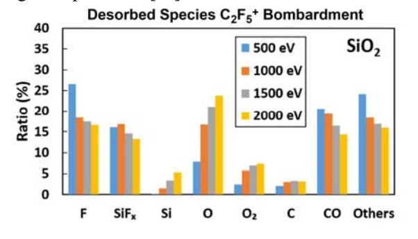
Figure 4-4: Fundamental Plasma-Surface Interactions by Molecular Dynamics. The interaction of plasma activated species and sheath accelerated ions with wafers (and plasma facing surfaces in the chamber) is at the heart of semiconductor fabrication. Molecular dynamics (MD) simulation is a first principles technique able to derive fundamental reaction probabilities and products, and predict the evolution of small features. The top image shows MD results for Si and \text{SiO}_2 after bombardment by 500 eV \text{NF}_2^+ and \text{C}_2\text{F}_5^+ ions. The bottom image shows the desorbed products following \text{C}_2\text{F}_5^+ bombardment of \text{SiO}_2 . Although MD requires inter-atomic potentials between all atoms in the system, which typically comes from other quantum-mechanical techniques, it is one of the few techniques to quantify mixing, implantation and synergistic interactions. A challenge for MD is scaling to large enough spatial dimensions over long enough times to evaluate evolution of full features for complex materials. [Images adapted from [69].
