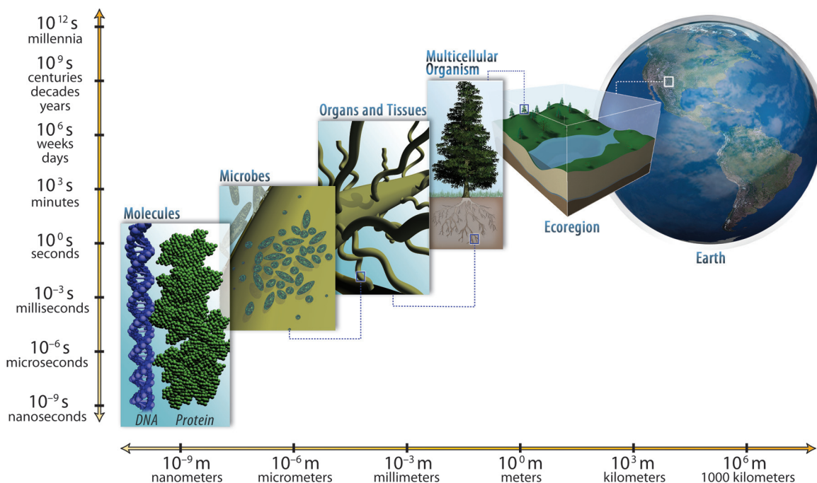
Fig. 1.1. Investigating Biological and Environmental Interactions Across Scales. Understanding how complex biological and environmental systems will respond to and affect critical Earth system processes requires measuring, simulating, and integrating biological, chemical, and physical components and their interactions across vast spatial and temporal scales—from subnanometers to kilometers and nanoseconds to millennia. Shown here is the example of moving from an initial view of molecules inside a cell, to cellular components, whole cells, the cells of a tissue interacting with adjacent cells, the tissue as part of an organism (e.g., a tree), the organism within a geographical region of a continent, and finally to a view of the whole Earth. As computational models become refined and increasingly precise at each scale, the question of how a model can interact meaningfully with those at adjacent scales will present opportunities to gain a deeper system understanding. [Image from p. 46 of the Grand Challenges for Biological and Environmental Research: A Long-Term Vision report.]
