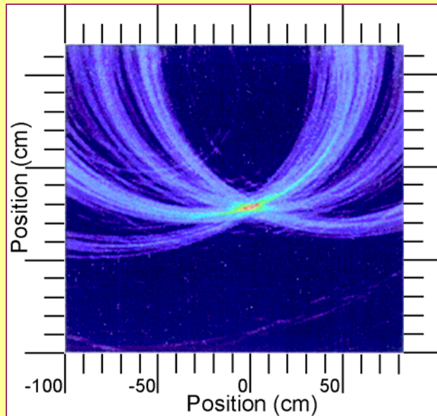
Compton circles from the gamma-ray tracking system at the Naval Research Laboratory. Source is located 120 cm from the detectors.
