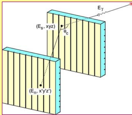
Schematic layout of gamma-ray tracking system
